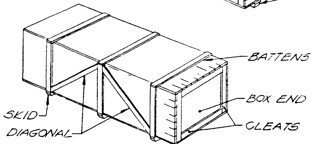
FIGURE 12. EXAMPLES OF REINFORCED STYLE 2 BOXES
