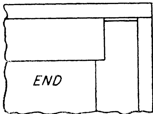
FIGURE 3. STYLE 2 \frac{1}{2} BOX (FULL CLEATED ENDS; NOTCHED CORNERS)
